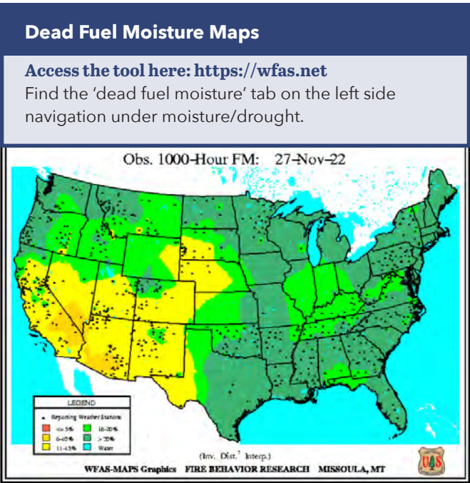
Image 7.13. Map of the observed 1,000 hour fuel moisture.
