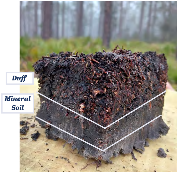
Image 7.10. Cubic soil sample, showing roots growing into the partly decomposed material (duff) on the forest floor. Image courtesy of Mac Callahan.
