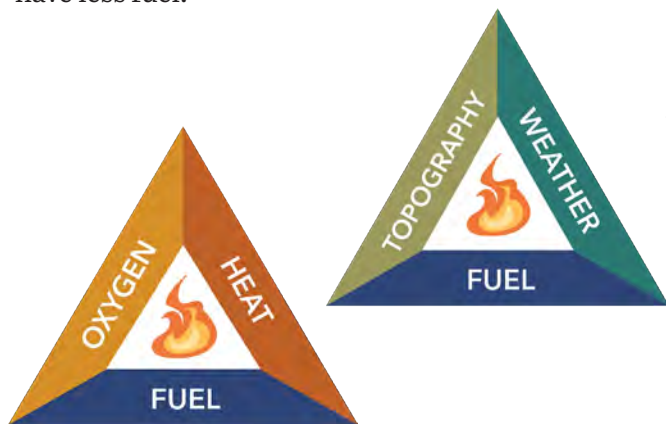
Figure 3.5. Fire Triangle & Fire Behavior Triangle. Learn more in Sections 7 & 8, Fuels & Fire Behavior.
