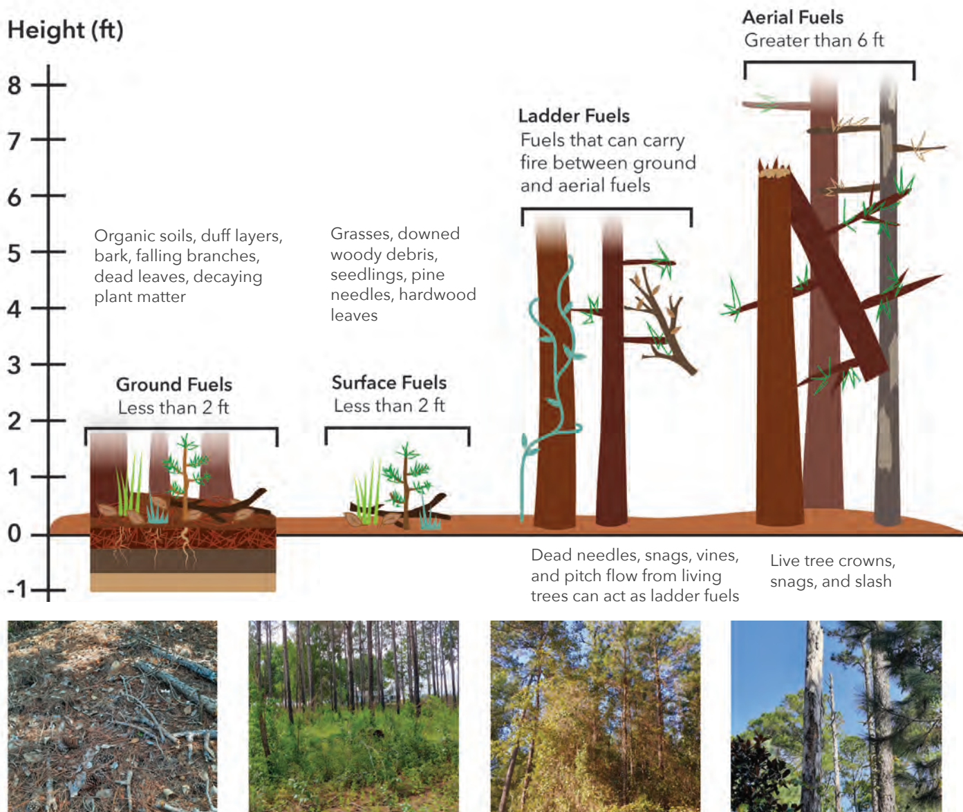
Figure 7.3. Diagram of vertical live and dead fuel classifications with example photos. Images courtesy of David Clabo.
