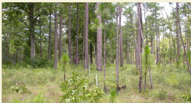
Figure 4.9. Photo time series of herbaceous vegetation changes starting immediately after the burn up to two years later. Images courtesy of Kevin Robertson.
