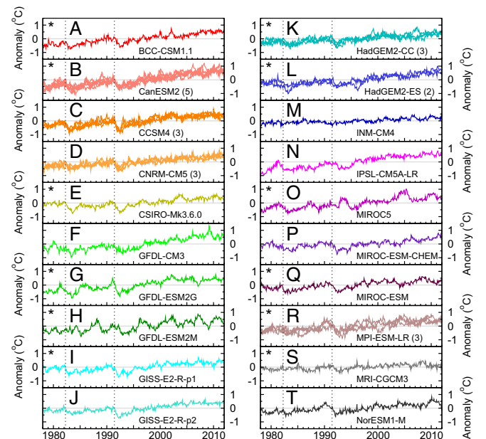
Fig. 2. The same as for Fig. 1, but for monthly mean anomalies in TLT. Results are from spliced historical/RCP8.5 simulations performed with 20 individual CMIP-5 models (panels A–T). Model anomalies are averaged over 82.5°N to 70°S.
