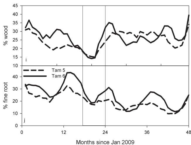
Extended Data Figure 5 | Impact of drought on carbon allocation for individual plots. This figure shows similar trends to those in Fig. 2, but with all the plots separated and extended for a further year for Tambopata and Kenia. a–d , Four years of total NPP ( \text{Mg C ha}^{-1} per month) (a), percentage allocation to canopy (b), percentage allocation to wood (c) and percentage allocation to fine roots (d) for the two plots in Kenia, Bolivia (black line, Kenia-A; grey line, Kenia-B). e–h , Seasonally detrended anomaly data for the same variables.
